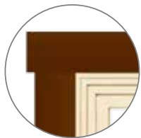
Flat trim with extended head
